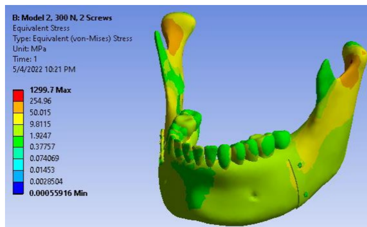
Figure 3: A) The overall tension distribution model of mandible with one miniplate on the right side and two bicortical screws on the left side (Loading force of 300 N on the first molars)
